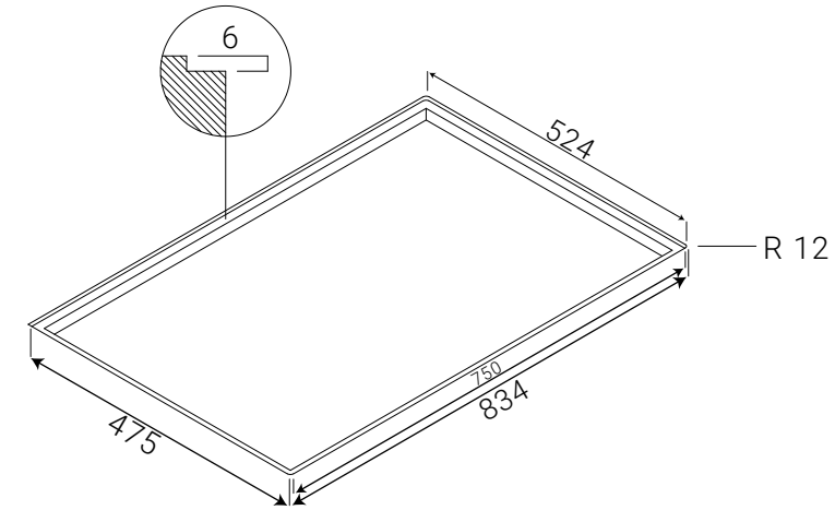
Flush Mounting
